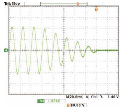
▲Fall time control waveform (example)
