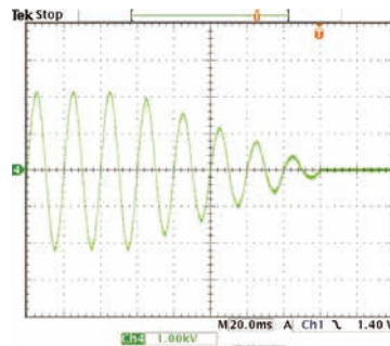
▲Fall time control waveform (example)
