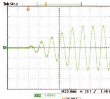
▲Rise time control waveform (example)
