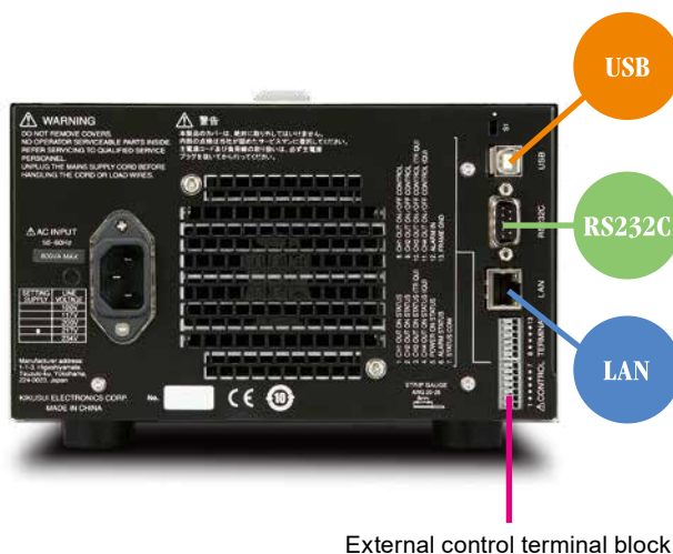
External control terminal block
