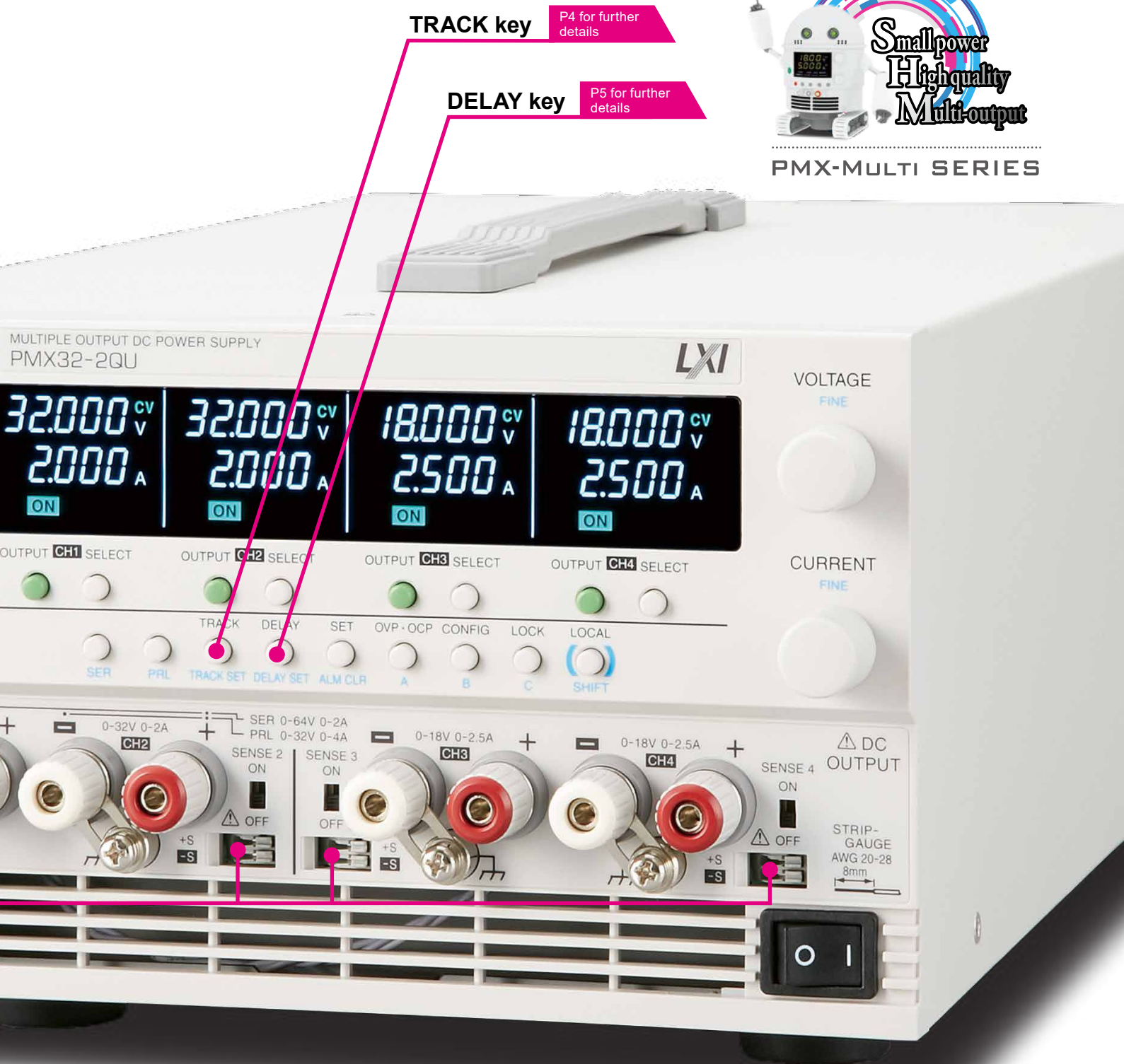
PMX32-2QU (four-output)
