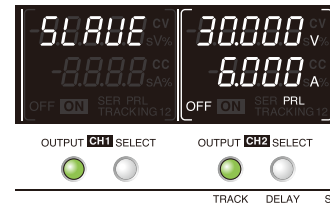
Panel display during parallel operation
