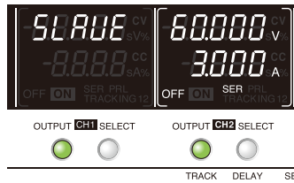
Panel display during series operation
