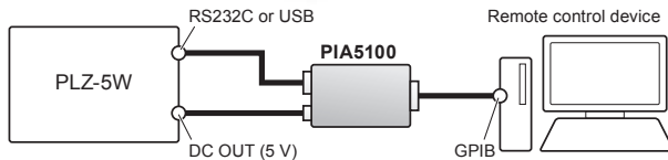
[Connection example]
