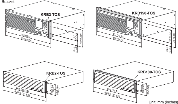
Bracket
